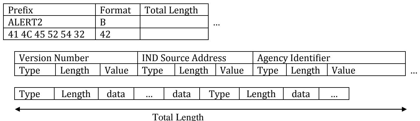
Figure 6-1 Asynchronous Binary Serial Interface structure
