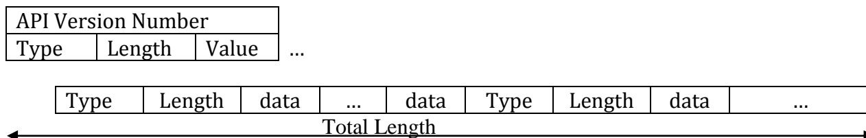
Figure 3-1 Asynchronous Binary Serial Interface form
